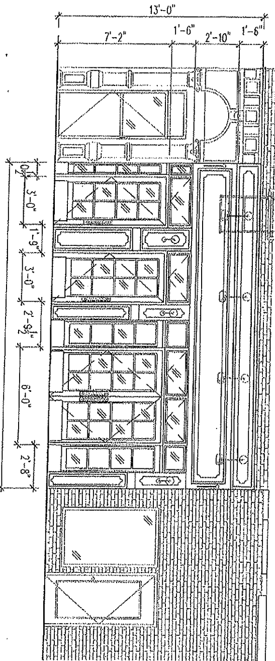
02 NINTH AVENUE ELEVATION
